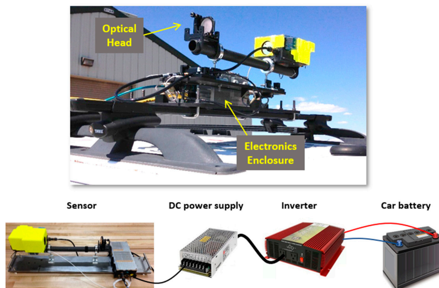
Figure 2. (Top): Photograph of sensor vehicle roof mount. (Bottom): Pictorial view of components used to power the sensor for vehicle deployments.
