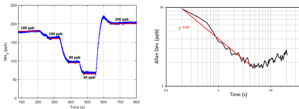
Figure 6. (Left): Comparison between measured and expected ammonia concentrations with closed-path configuration. Red bars show the fixed delivered concentrations. (Right): Allan variance analysis shows the sensitivity of \sim 4 ppb (at 1 s).
