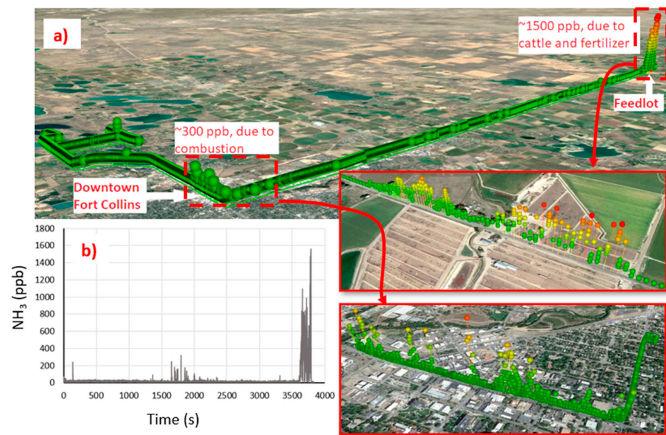
Figure 7. (a) Concentration data imported and viewed in Google Earth. (b) Ammonia concentration time series from the same data (~1 h measurement).
