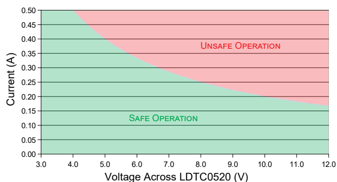
Figure 33. Laser Driver SOA Chart, LDT0520
