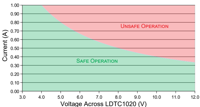
Figure 34. Laser Driver SOA Chart, LDT1020
